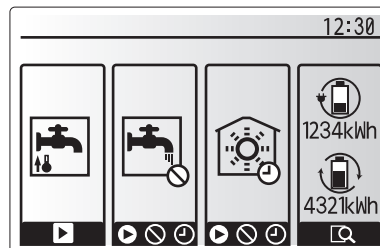
Option screen
